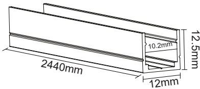
LB53538 - Aluminum Profile
