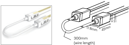
LB53536 - Coupling
