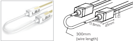
LB53536 - Coupling
