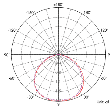
Light Distribution Curve (3000K, 120°)
