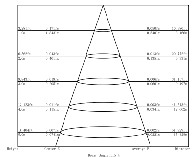
Lux distance Curve (3000K, 120°)
