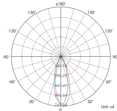
Light Distribution Curve (3000K, 36° COB reflector)
