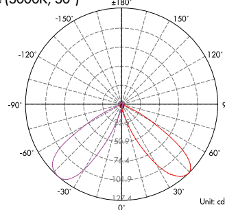
Light Distribution Curve (3000K, 30°)
